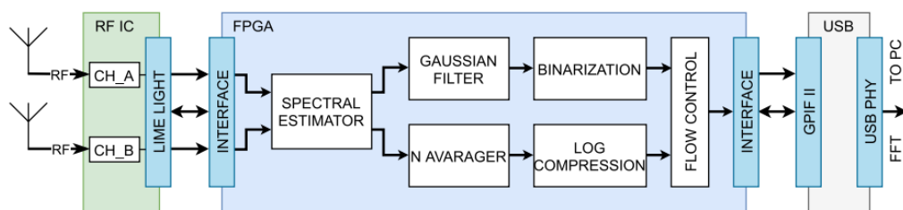
Figure 2 (sensor architecture based on SDR with extended FPGA) (Flak, 2021)
