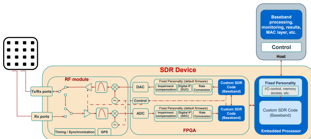
Figure 5 (FPGA-integrated SDR with MIMO capabilities) (Michailidis et al., 2024)
