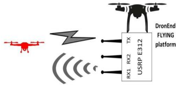
Figure 3 (DronEnd FLYING platform) (Chiper et al., 2022)
